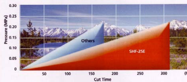
Comparison of Filter Life (SHF-25E vs. Other EDM Filters)
